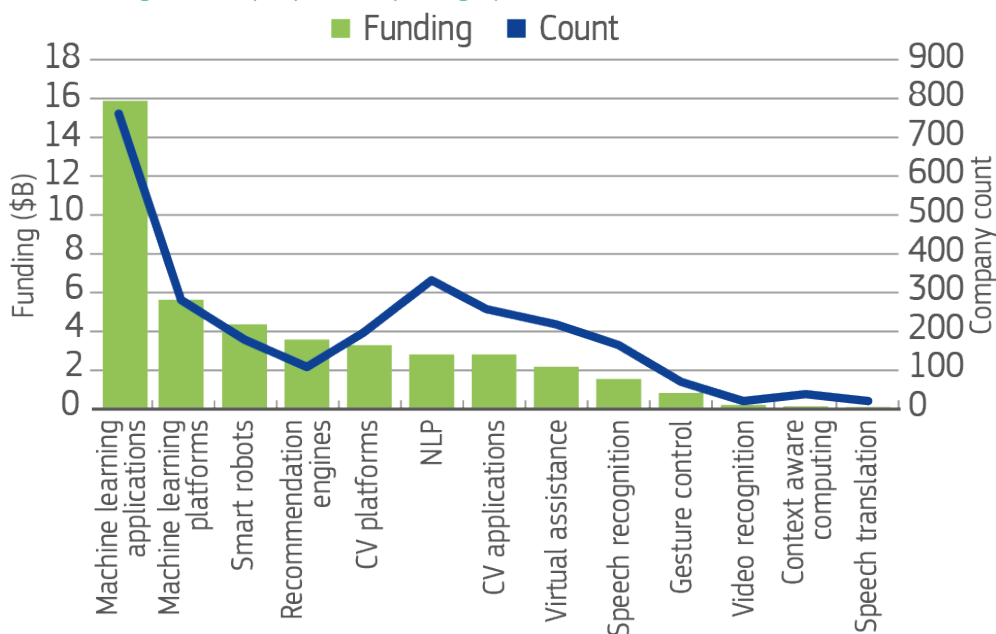
Graph 16: Artificial Intelligence
